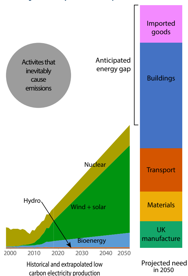
Figure 1.1: Gap between today and Absolute Zero
